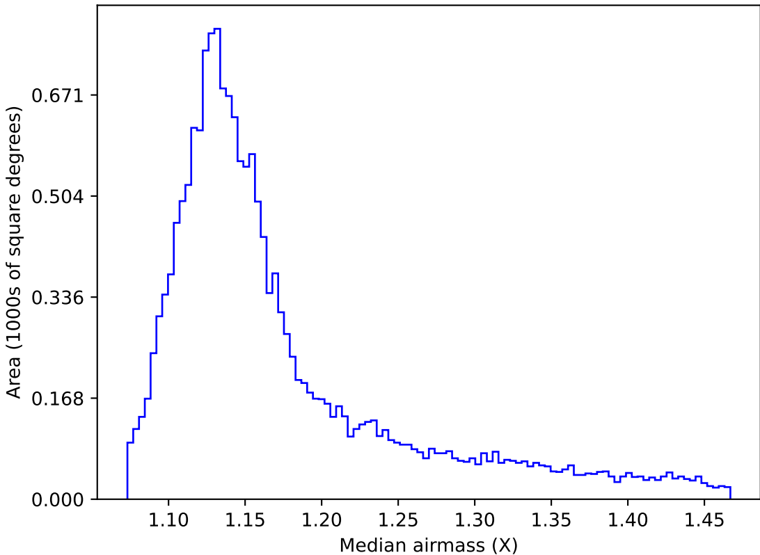
too_elab_r16_d2_ugrizy_v3.4_10yrs WFD r band: Median airmass
