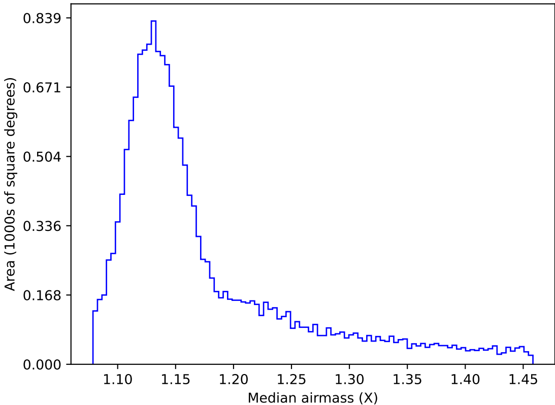
too_elab_r16_d2_ugrizy_v3.4_10yrs WFD i band: Median airmass
