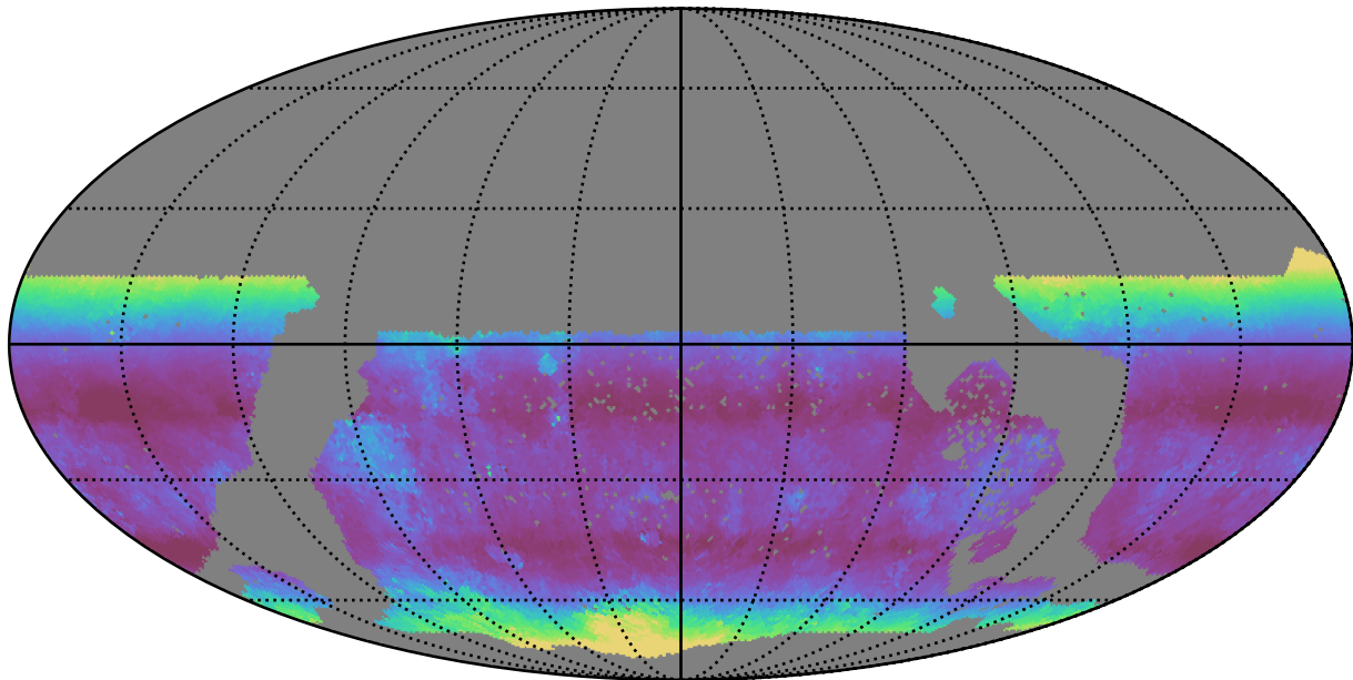
too_elab_r16_d2_ugrizy_v3.4_10yrs WFD g band: Median airmass
