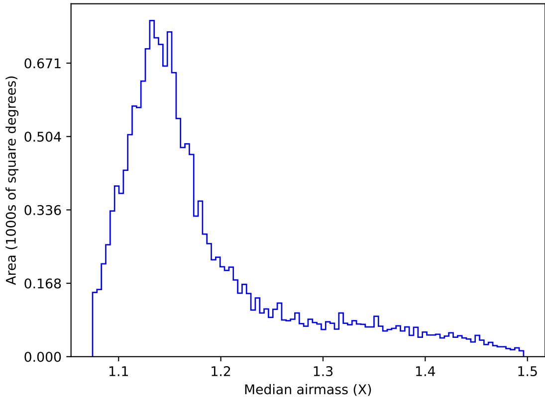
too_elab_r16_d2_ugrizy_v3.4_10yrs WFD g band: Median airmass
