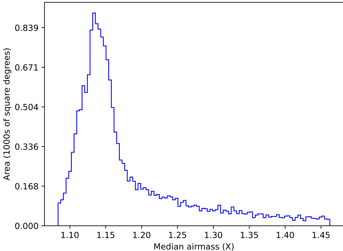
too_elab_r16_d2_ugrizy_v3.4_10yrs WFD all bands: Median airmass
