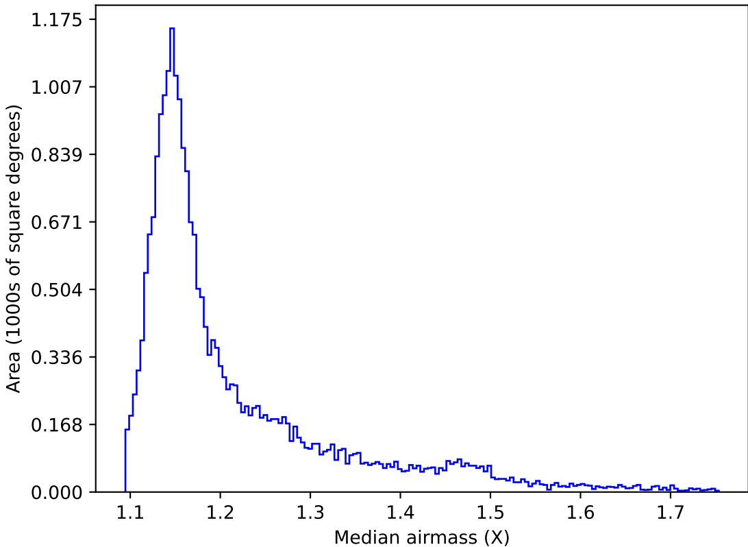
too_elab_r16_d2_ugrizy_v3.4_10yrs All sky y band: Median airmass
