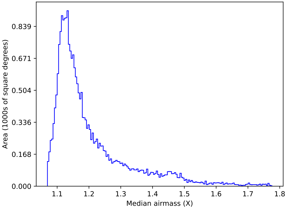
too_elab_r16_d2_ugrizy_v3.4_10yrs All sky u band: Median airmass
