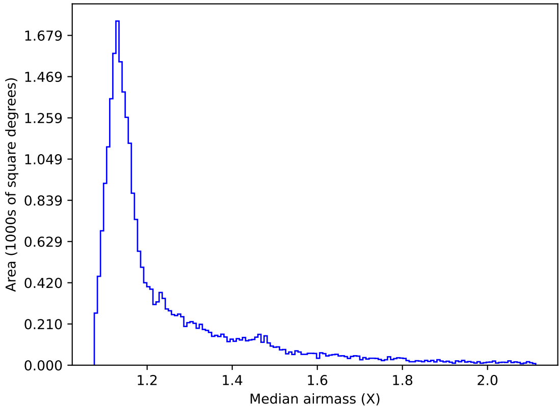
too_elab_r16_d2_ugrizy_v3.4_10yrs All sky r band: Median airmass
