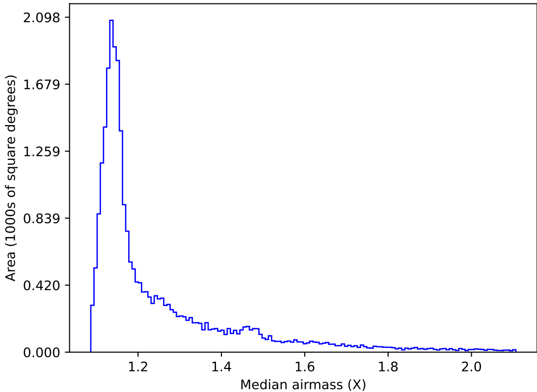
too_elab_r16_d2_ugrizy_v3.4_10yrs All sky all bands: Median airmass
