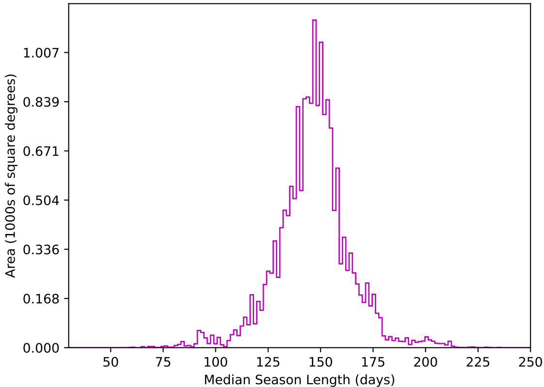
too_elab_r16_d2_ugrizy_v3.4_10yrs WFD z band: Median Season Length
