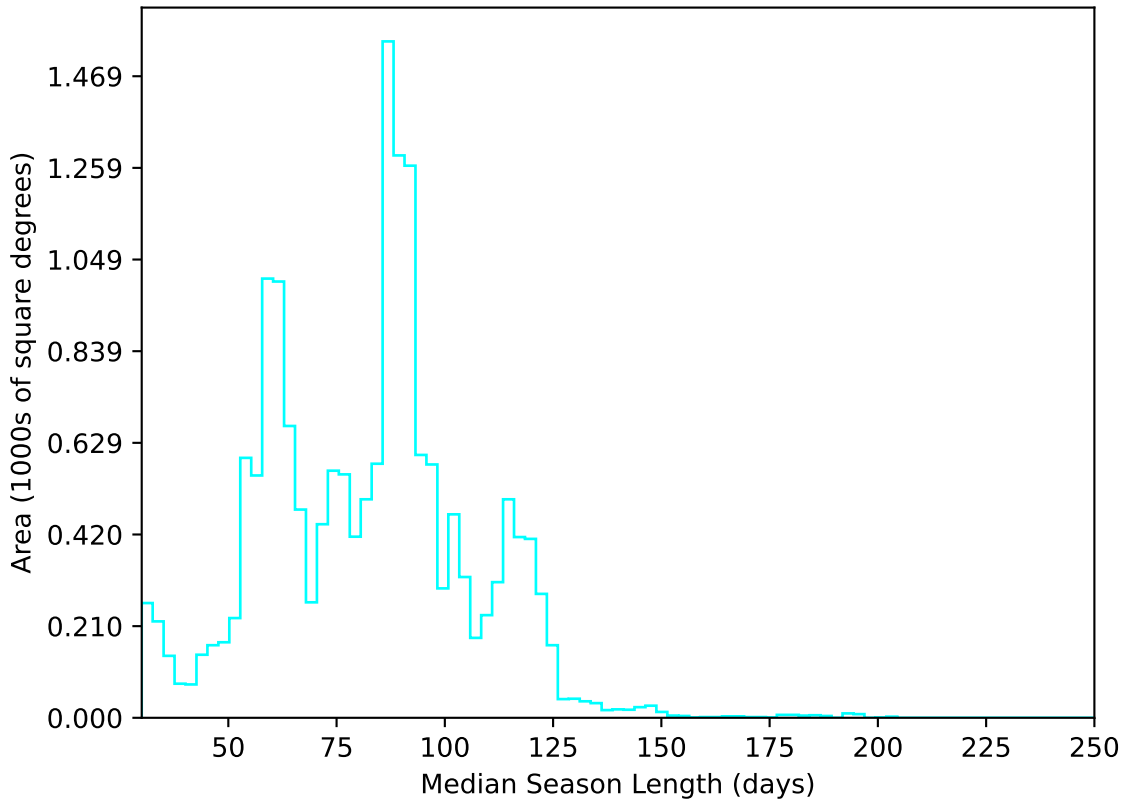
too_elab_r16_d2_ugrizy_v3.4_10yrs WFD u band: Median Season Length
