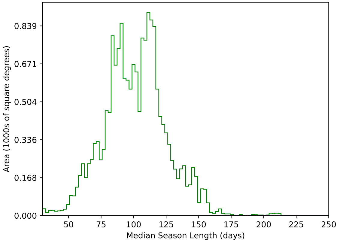
too_elab_r16_d2_ugrizy_v3.4_10yrs WFD g band: Median Season Length
