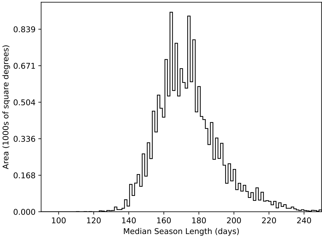
too_elab_r16_d2_ugrizy_v3.4_10yrs WFD all bands: Median Season Length
