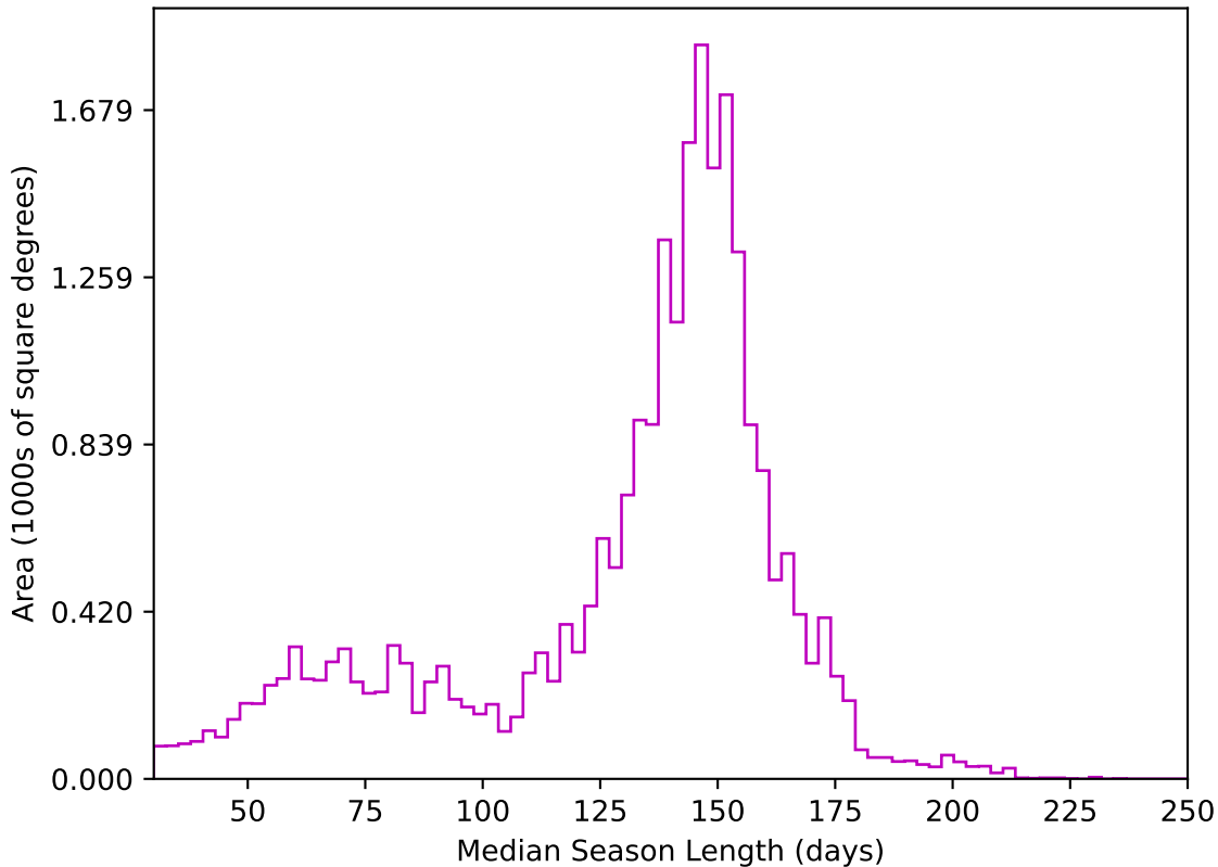
too_elab_r16_d2_ugrizy_v3.4_10yrs All sky z band: Median Season Length
