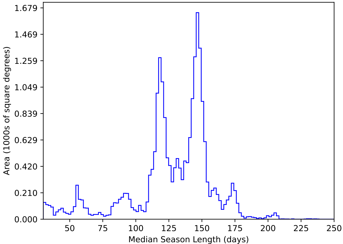
too_elab_r16_d2_ugrizy_v3.4_10yrs All sky y band: Median Season Length
