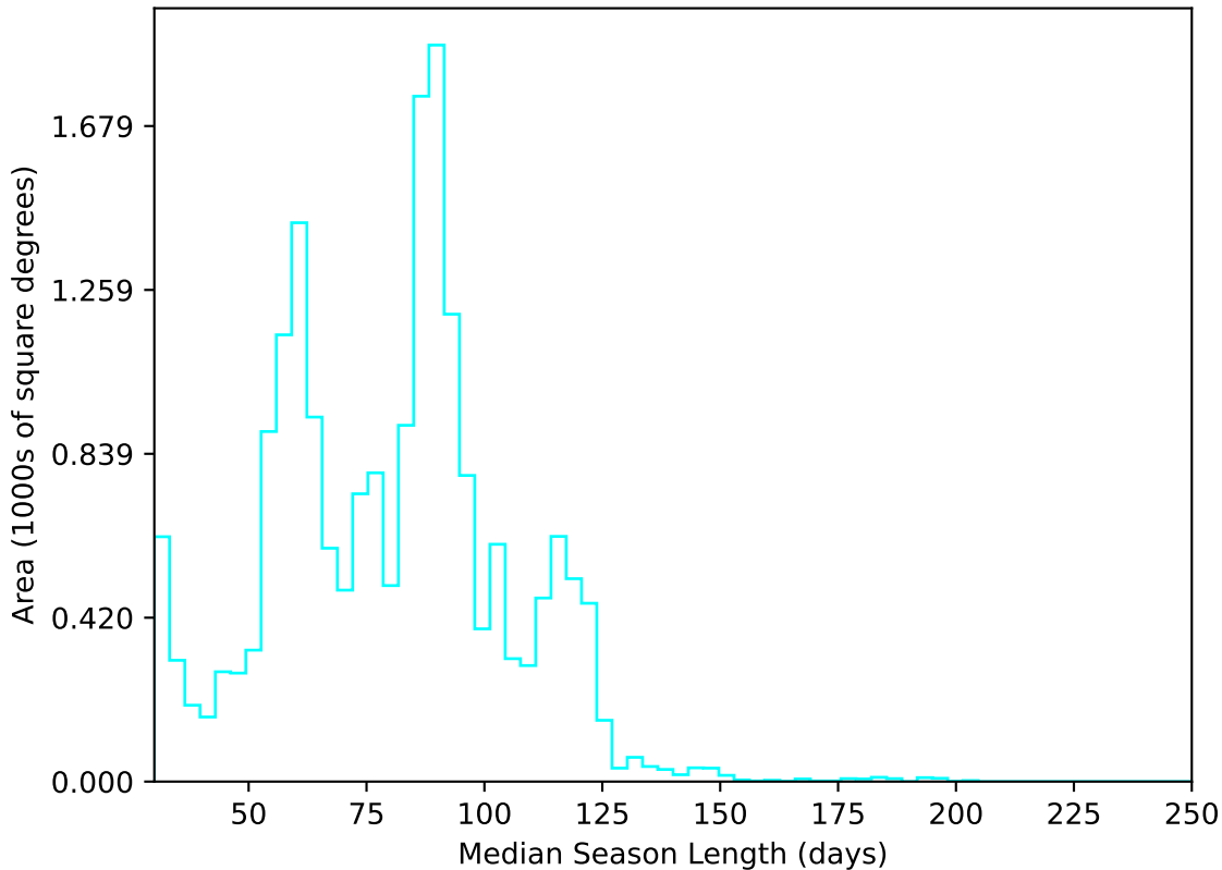
too_elab_r16_d2_ugrizy_v3.4_10yrs All sky u band: Median Season Length
