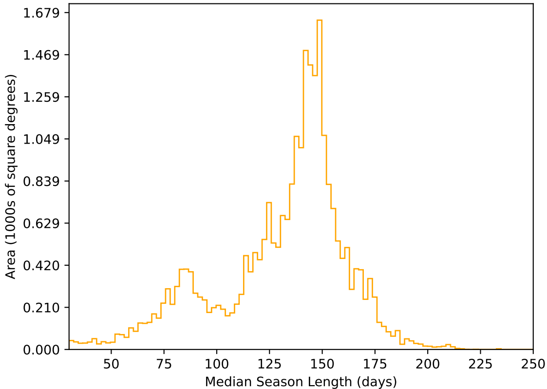
too_elab_r16_d2_ugrizy_v3.4_10yrs All sky r band: Median Season Length
