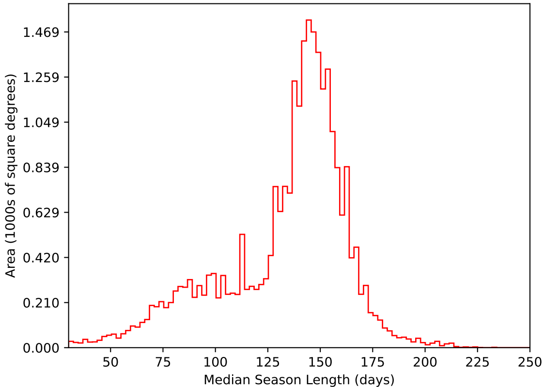
too_elab_r16_d2_ugrizy_v3.4_10yrs All sky i band: Median Season Length
