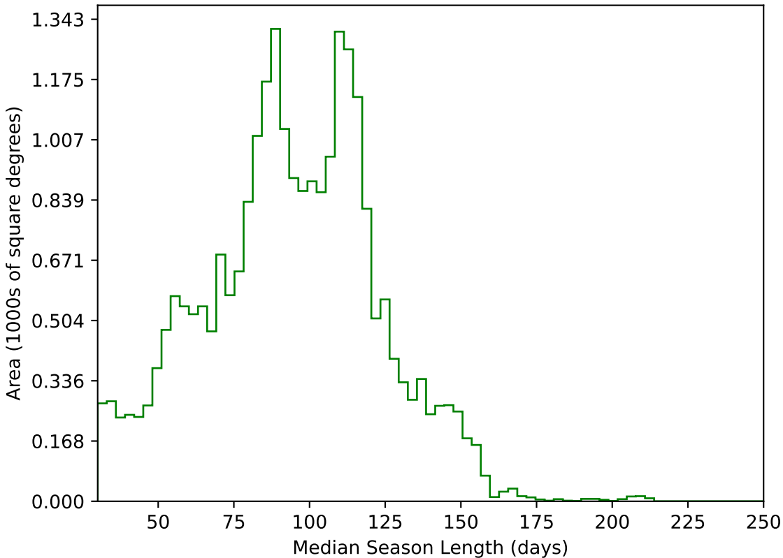
too_elab_r16_d2_ugrizy_v3.4_10yrs All sky g band: Median Season Length
