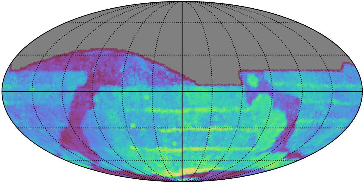
too_elab_r16_d2_ugrizy_v3.4_10yrs All sky all bands: Median Season Length
