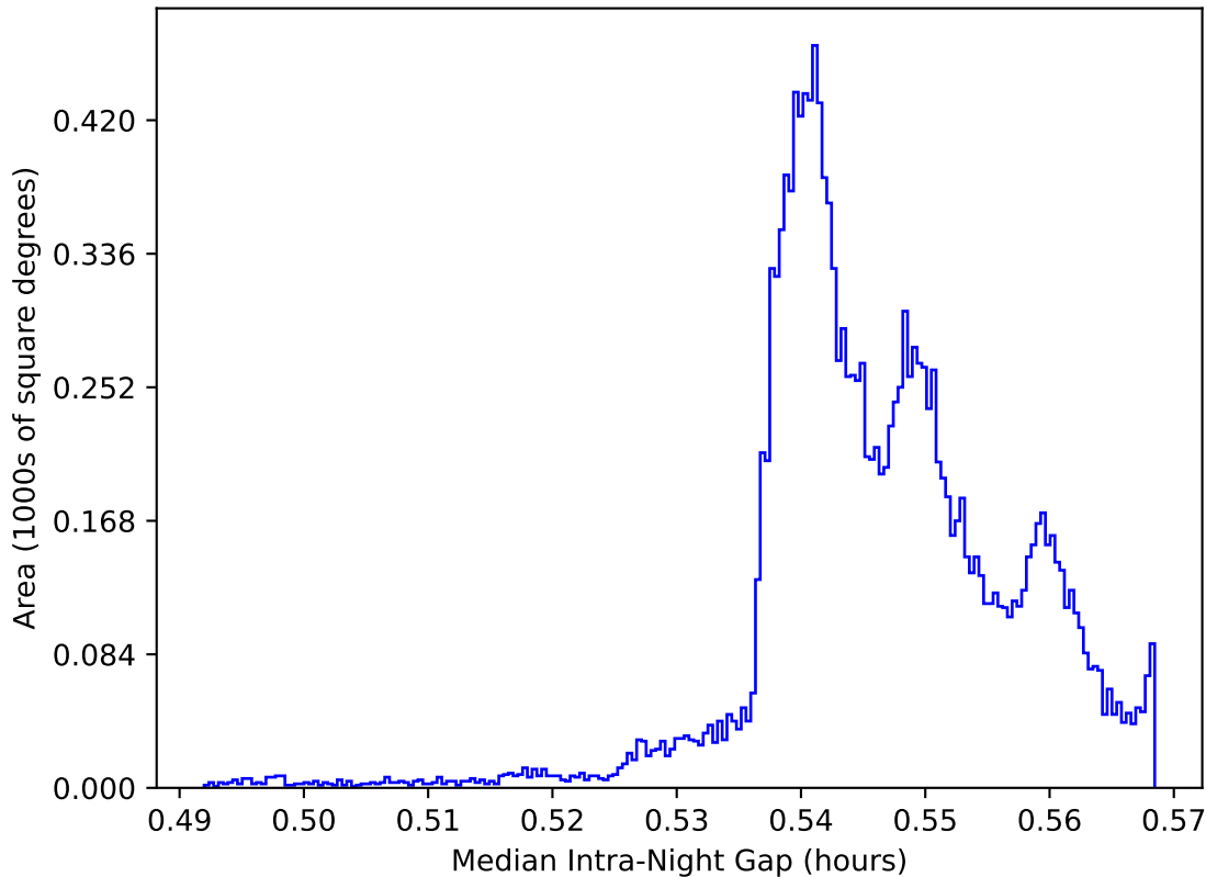
too_elab_r16_d2_ugrizy_v3.4_10yrs WFD: Median Intra-Night Gap
