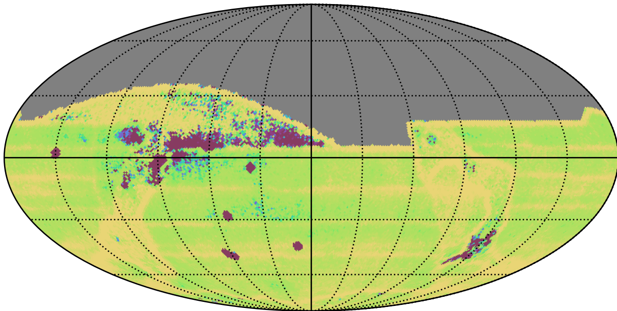
too_elab_r16_d2_ugrizy_v3.4_10yrs All sky: Median Intra-Night Gap
