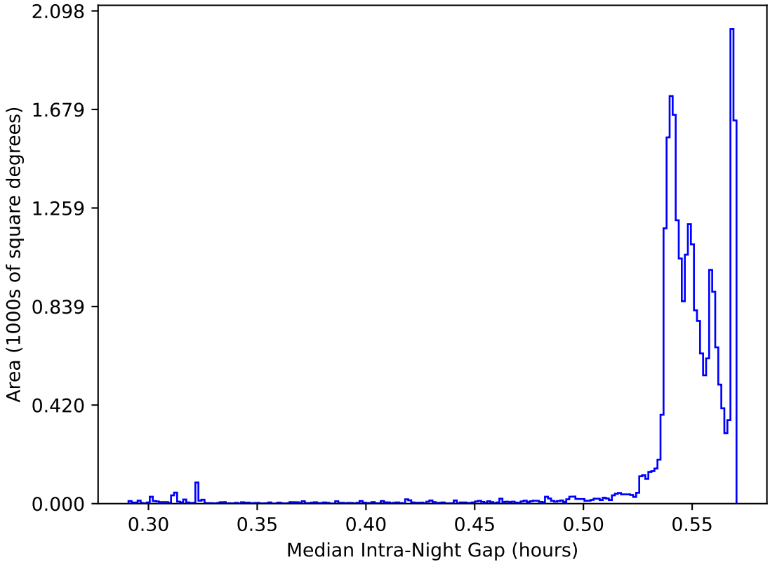
too_elab_r16_d2_ugrizy_v3.4_10yrs All sky: Median Intra-Night Gap
