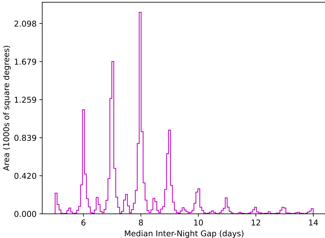
too_elab_r16_d2_ugrizy_v3.4_10yrs WFD z band: Median Inter-Night Gap
