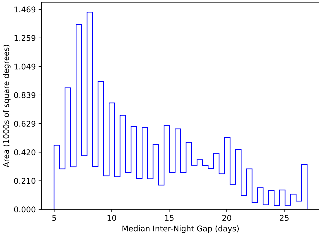
too_elab_r16_d2_ugrizy_v3.4_10yrs WFD y band: Median Inter-Night Gap
