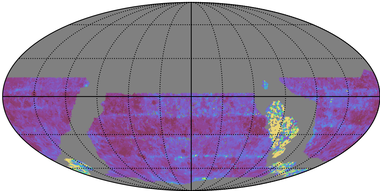
too_elab_r16_d2_ugrizy_v3.4_10yrs WFD u band: Median Inter-Night Gap
