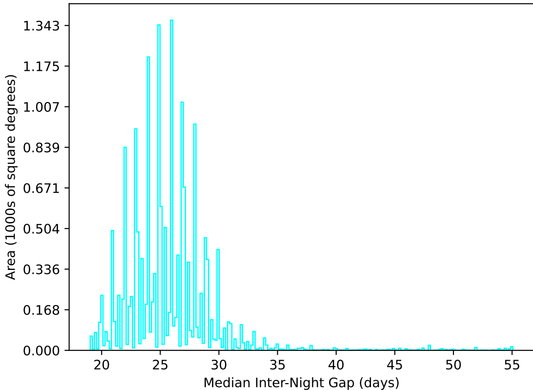
too_elab_r16_d2_ugrizy_v3.4_10yrs WFD u band: Median Inter-Night Gap
