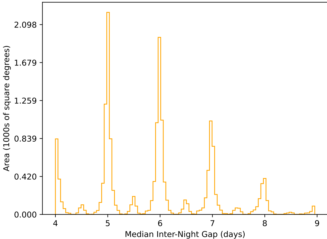
too_elab_r16_d2_ugrizy_v3.4_10yrs WFD r band: Median Inter-Night Gap
