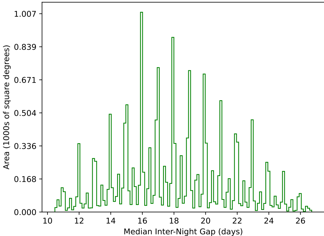
too_elab_r16_d2_ugrizy_v3.4_10yrs WFD g band: Median Inter-Night Gap
