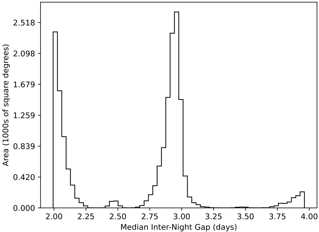
too_elab_r16_d2_ugrizy_v3.4_10yrs WFD all bands: Median Inter-Night Gap
