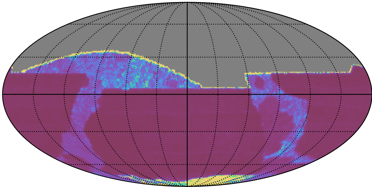
too_elab_r16_d2_ugrizy_v3.4_10yrs All sky z band: Median Inter-Night Gap
