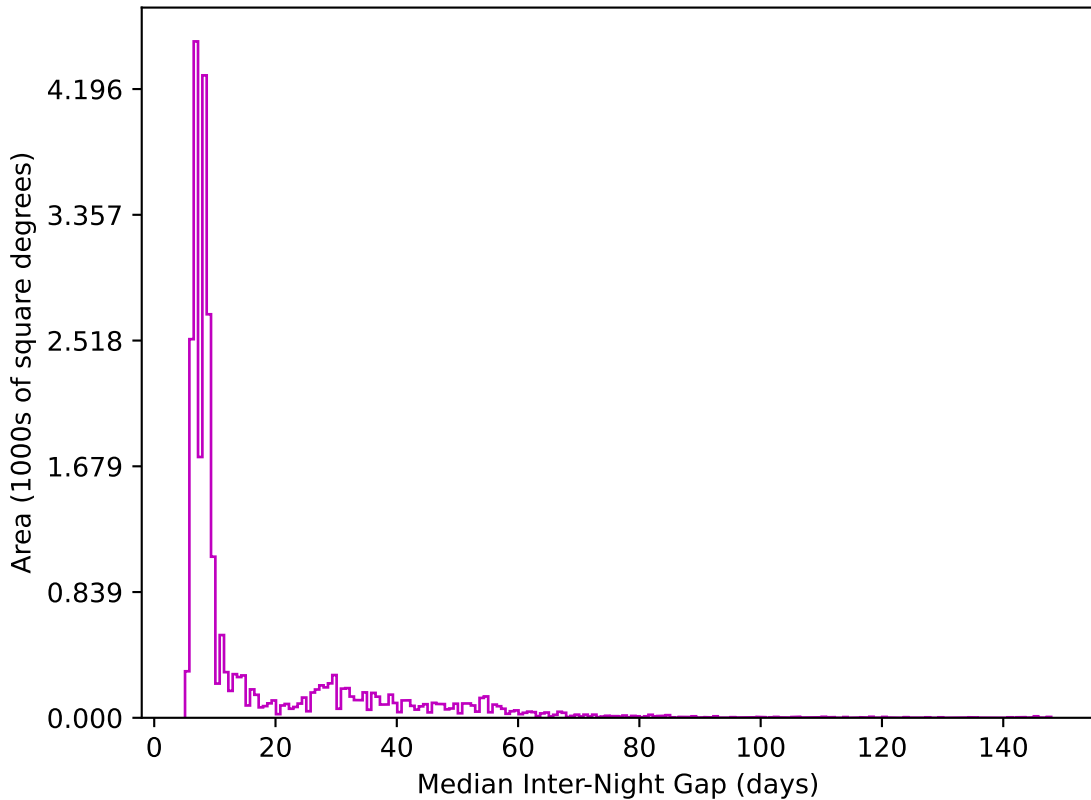
too_elab_r16_d2_ugrizy_v3.4_10yrs All sky z band: Median Inter-Night Gap
