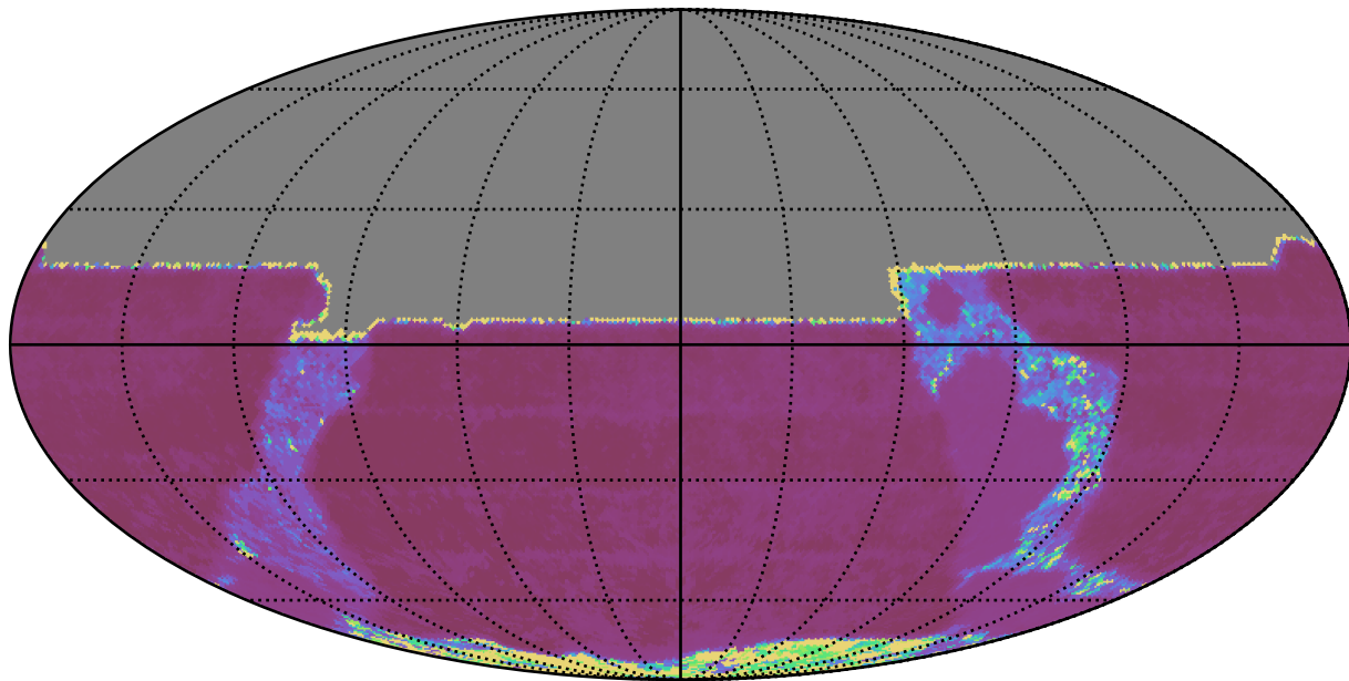
too_elab_r16_d2_ugrizy_v3.4_10yrs All sky y band: Median Inter-Night Gap
