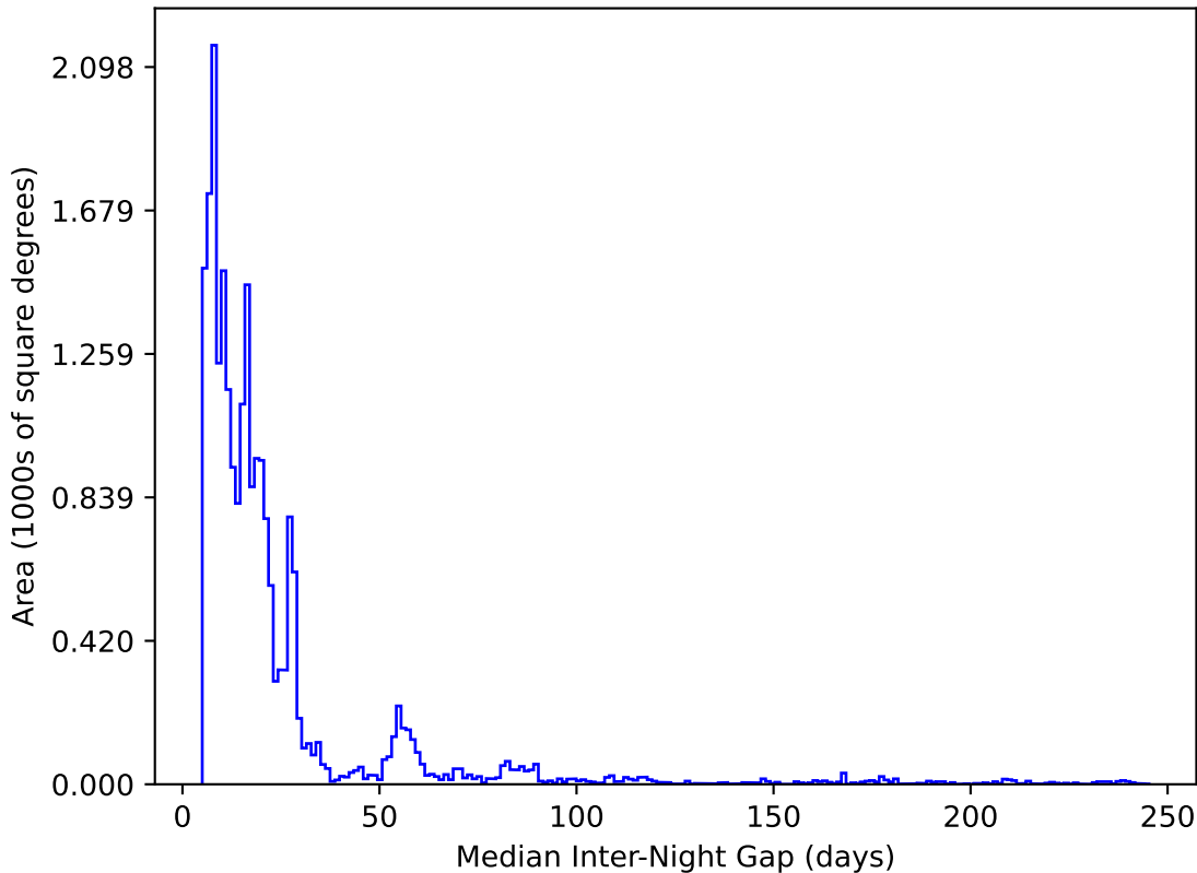
too_elab_r16_d2_ugrizy_v3.4_10yrs All sky y band: Median Inter-Night Gap
