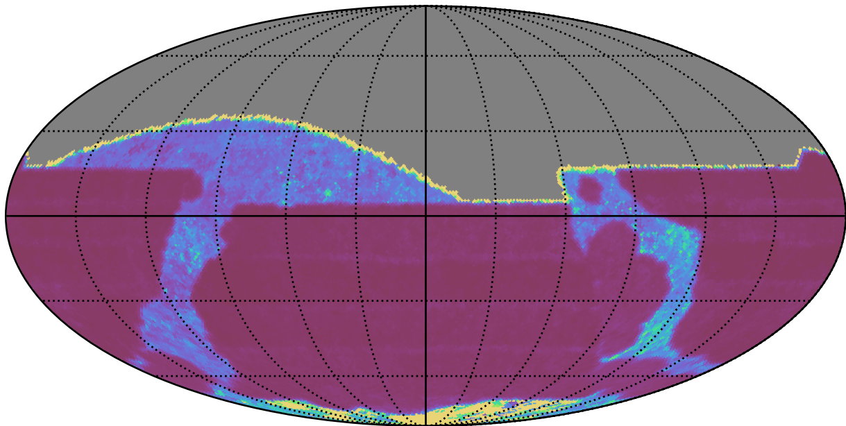
too_elab_r16_d2_ugrizy_v3.4_10yrs All sky r band: Median Inter-Night Gap
