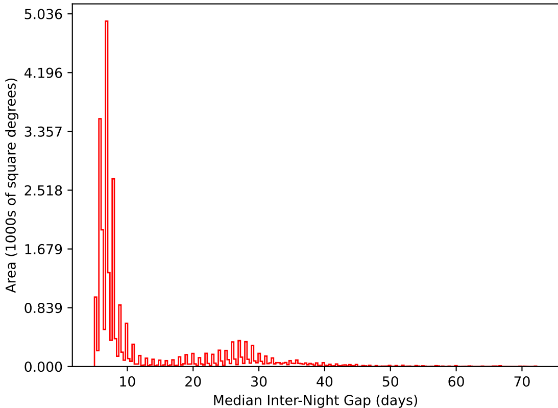
too_elab_r16_d2_ugrizy_v3.4_10yrs All sky i band: Median Inter-Night Gap
