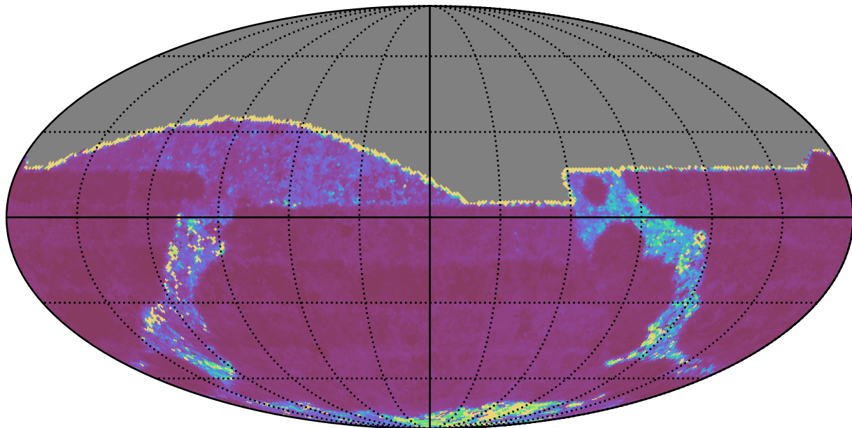
too_elab_r16_d2_ugrizy_v3.4_10yrs All sky g band: Median Inter-Night Gap
