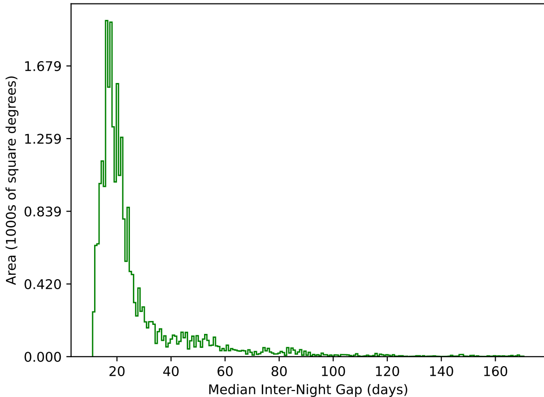
too_elab_r16_d2_ugrizy_v3.4_10yrs All sky g band: Median Inter-Night Gap
