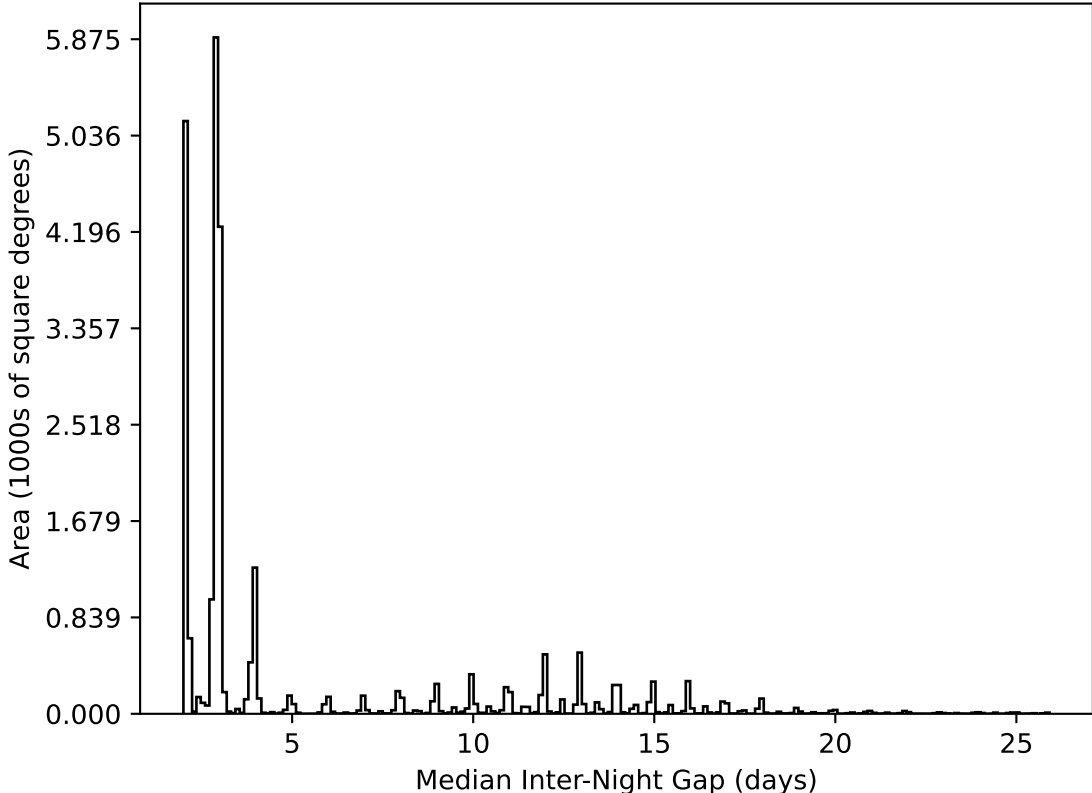
too_elab_r16_d2_ugrizy_v3.4_10yrs All sky all bands: Median Inter-Night Gap
