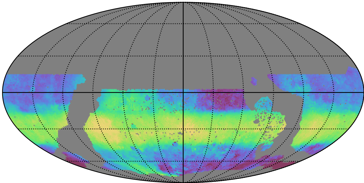
too_elab_r16_d2_ugrizy_v3.4_10yrs WFD z band: Median HA
