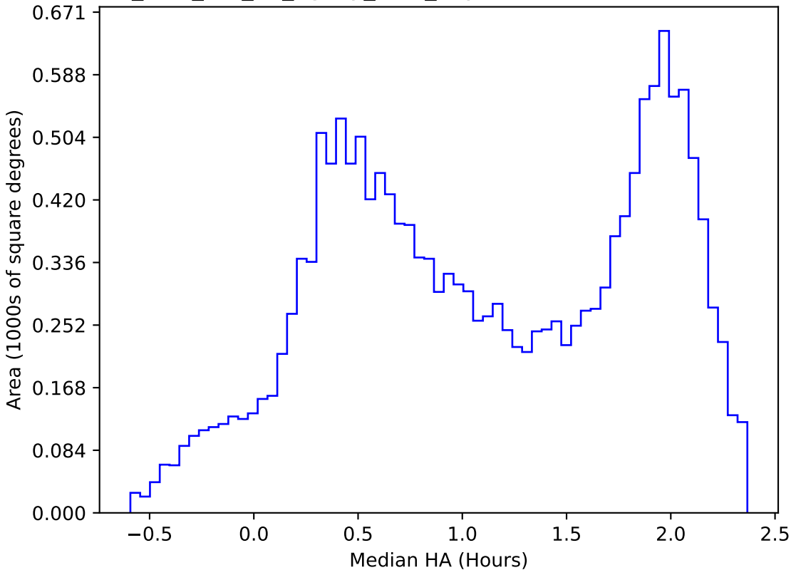
too_elab_r16_d2_ugrizy_v3.4_10yrs WFD z band: Median HA
