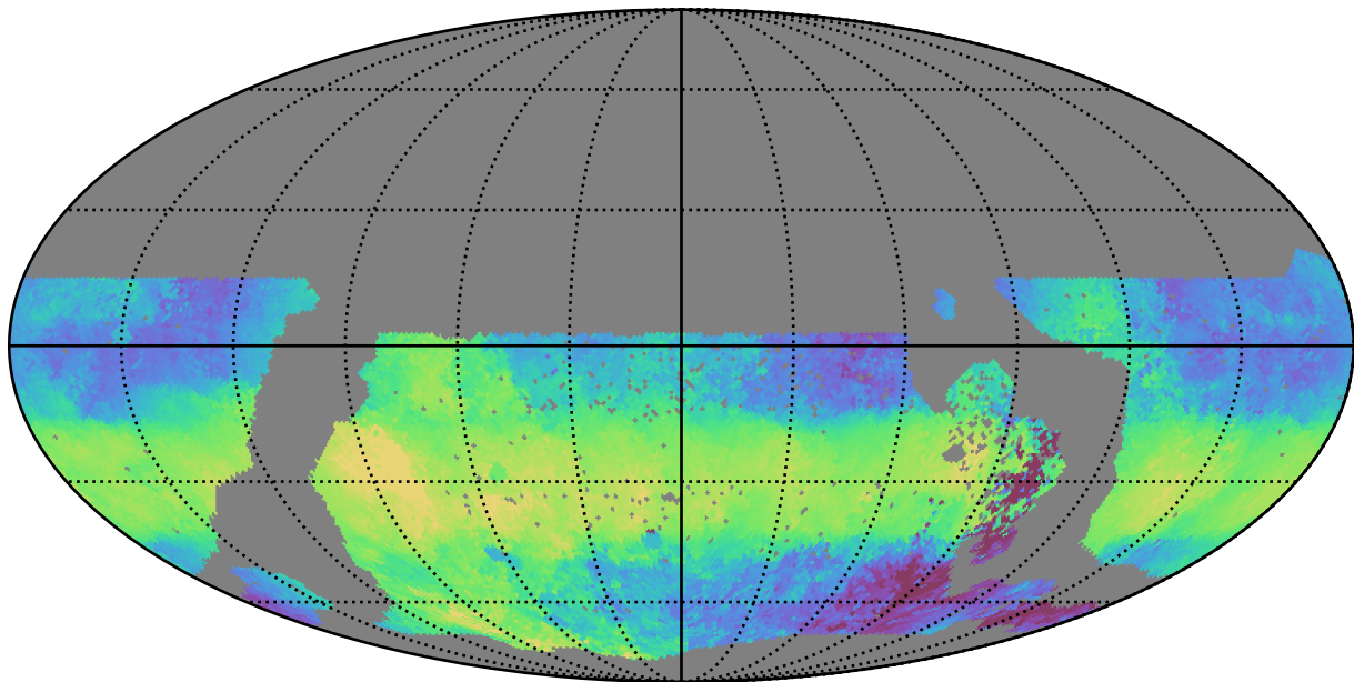
too_elab_r16_d2_ugrizy_v3.4_10yrs WFD u band: Median HA
