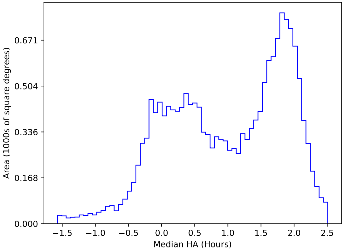
too_elab_r16_d2_ugrizy_v3.4_10yrs WFD u band: Median HA
