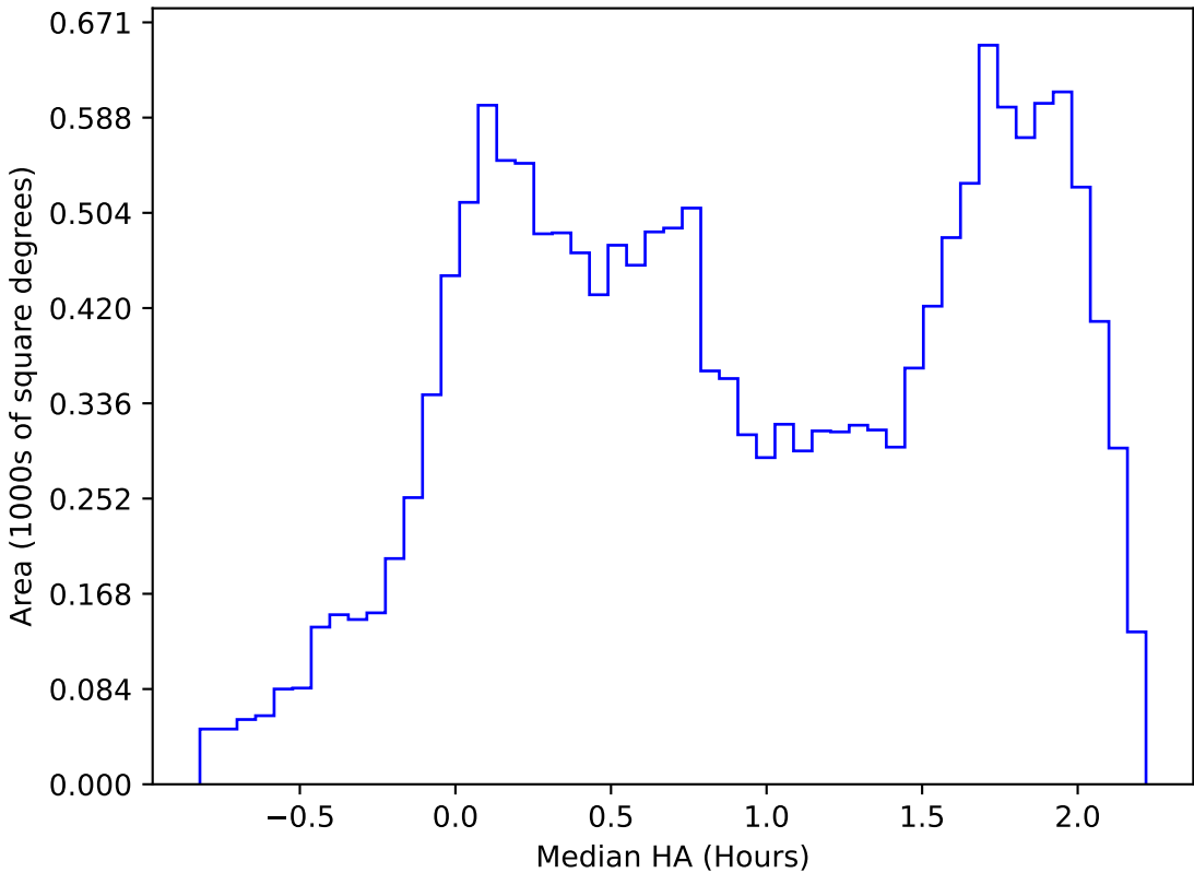
too_elab_r16_d2_ugrizy_v3.4_10yrs WFD r band: Median HA
