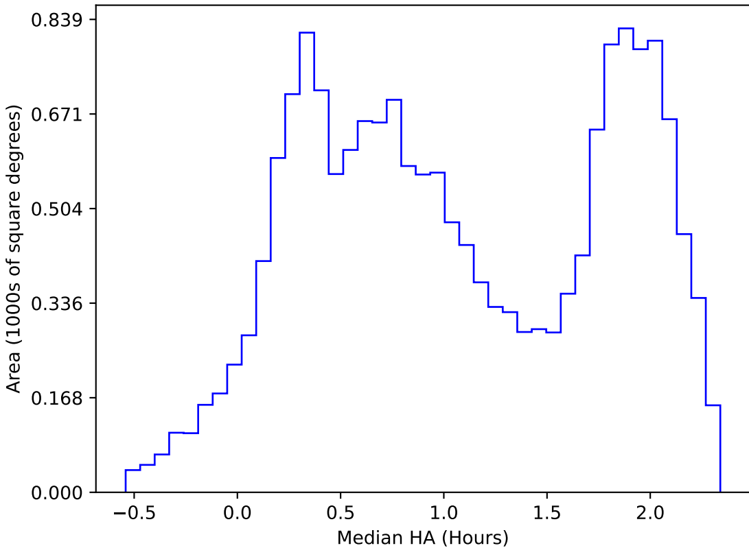
too_elab_r16_d2_ugrizy_v3.4_10yrs WFD i band: Median HA
