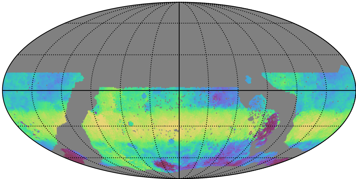
too_elab_r16_d2_ugrizy_v3.4_10yrs WFD g band: Median HA
