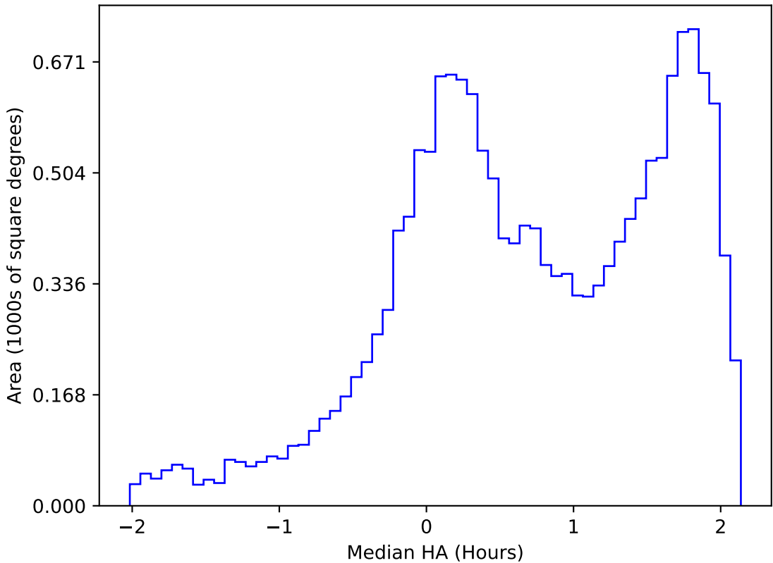
too_elab_r16_d2_ugrizy_v3.4_10yrs WFD g band: Median HA
