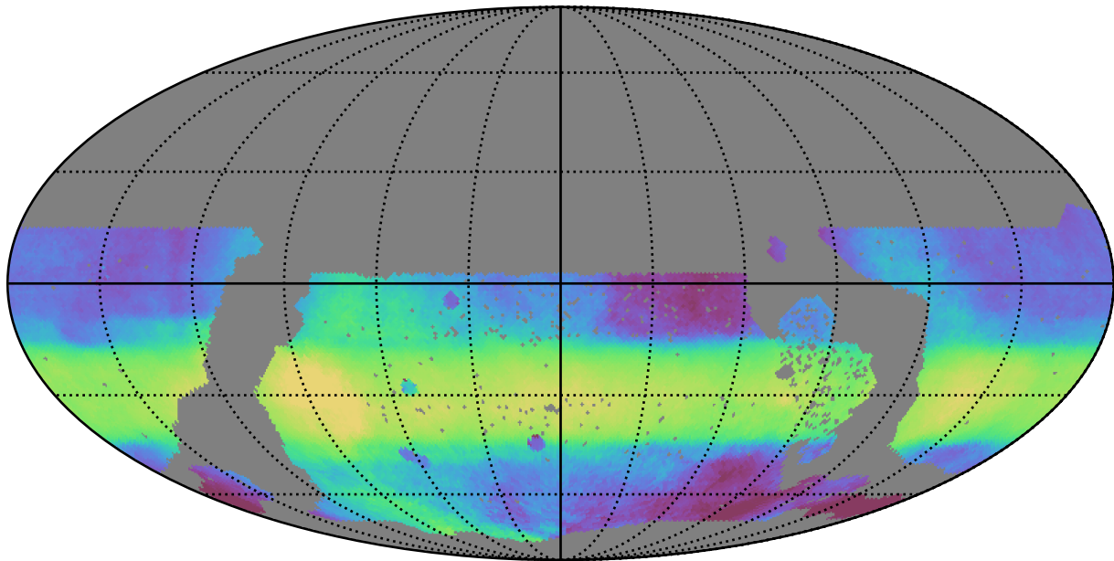
too_elab_r16_d2_ugrizy_v3.4_10yrs WFD all bands: Median HA
