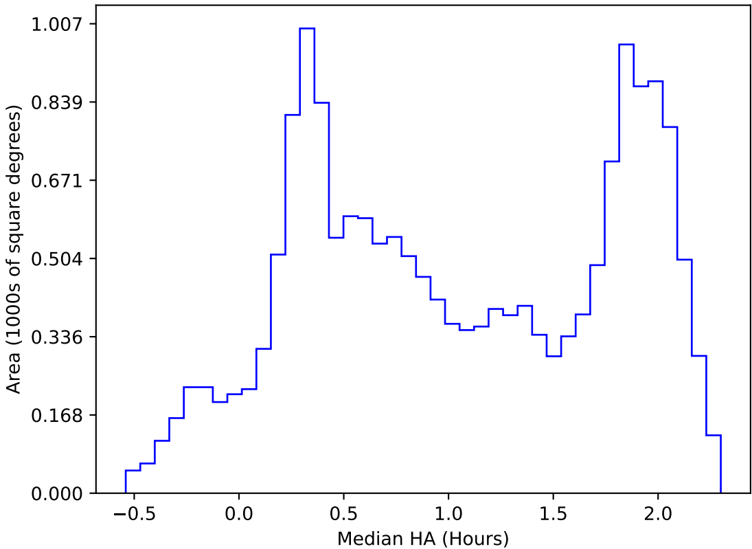
too_elab_r16_d2_ugrizy_v3.4_10yrs WFD all bands: Median HA
