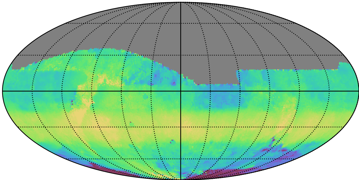
too_elab_r16_d2_ugrizy_v3.4_10yrs All sky z band: Median HA
